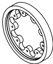
CLUTCH SPRING CENTERING TOOL
